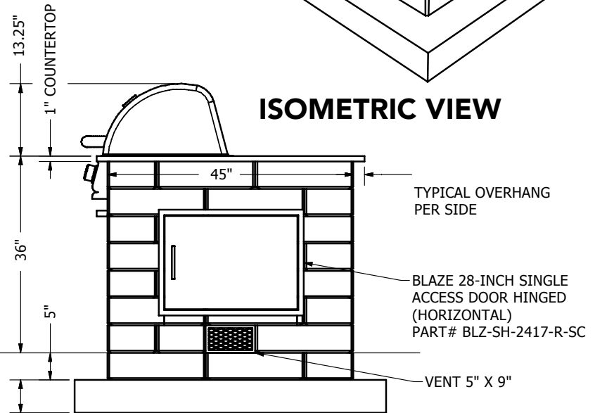
SIDE ELEVATION VIEW
