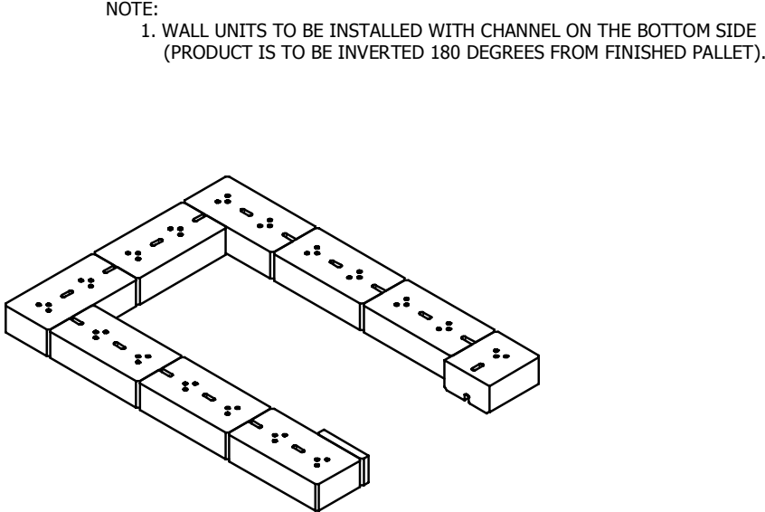
ISOMETRIC VIEW
