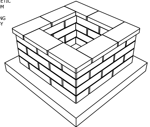
ISOMETRIC VIEW
