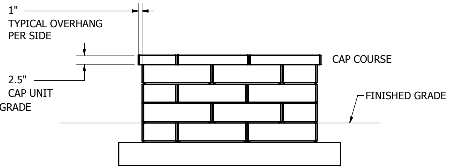
SIDE ELEVATION VIEW
